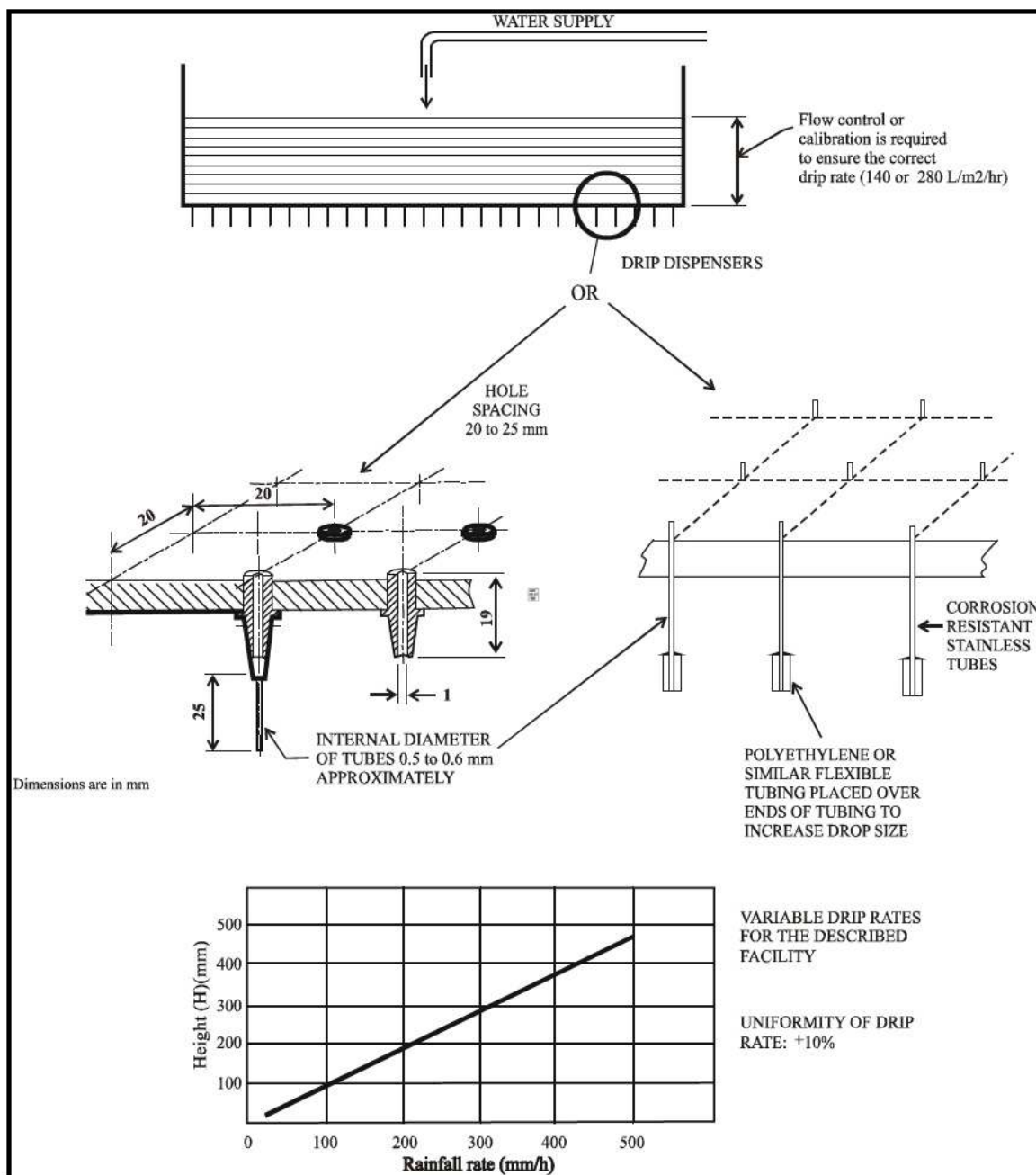
Figure 506.6-1. Sample facility for steady state rain or drip test.
